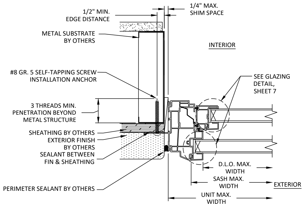
B 4 HORIZONTAL SECTION NAIL FIN INSTALLATION METAL SUBSTRATE
