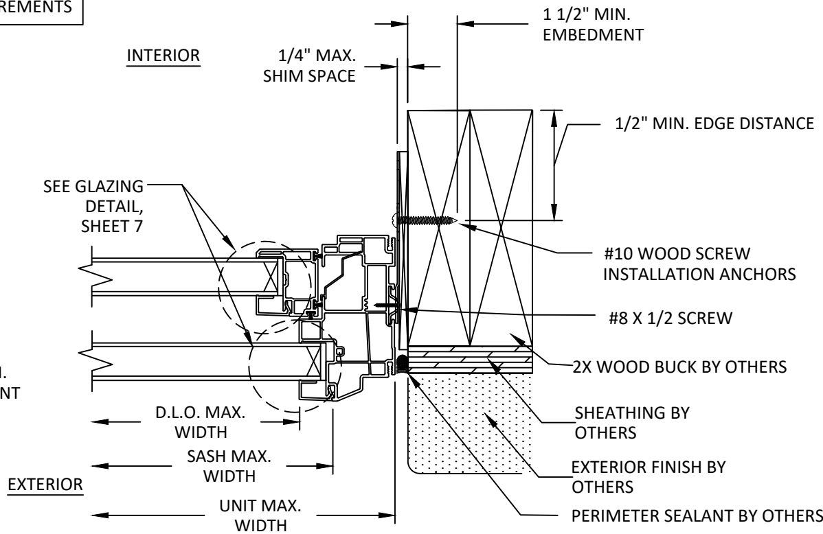
D 6 HORIZONTAL SECTION CLIP INSTALLATION WOOD SUBSTRATE
