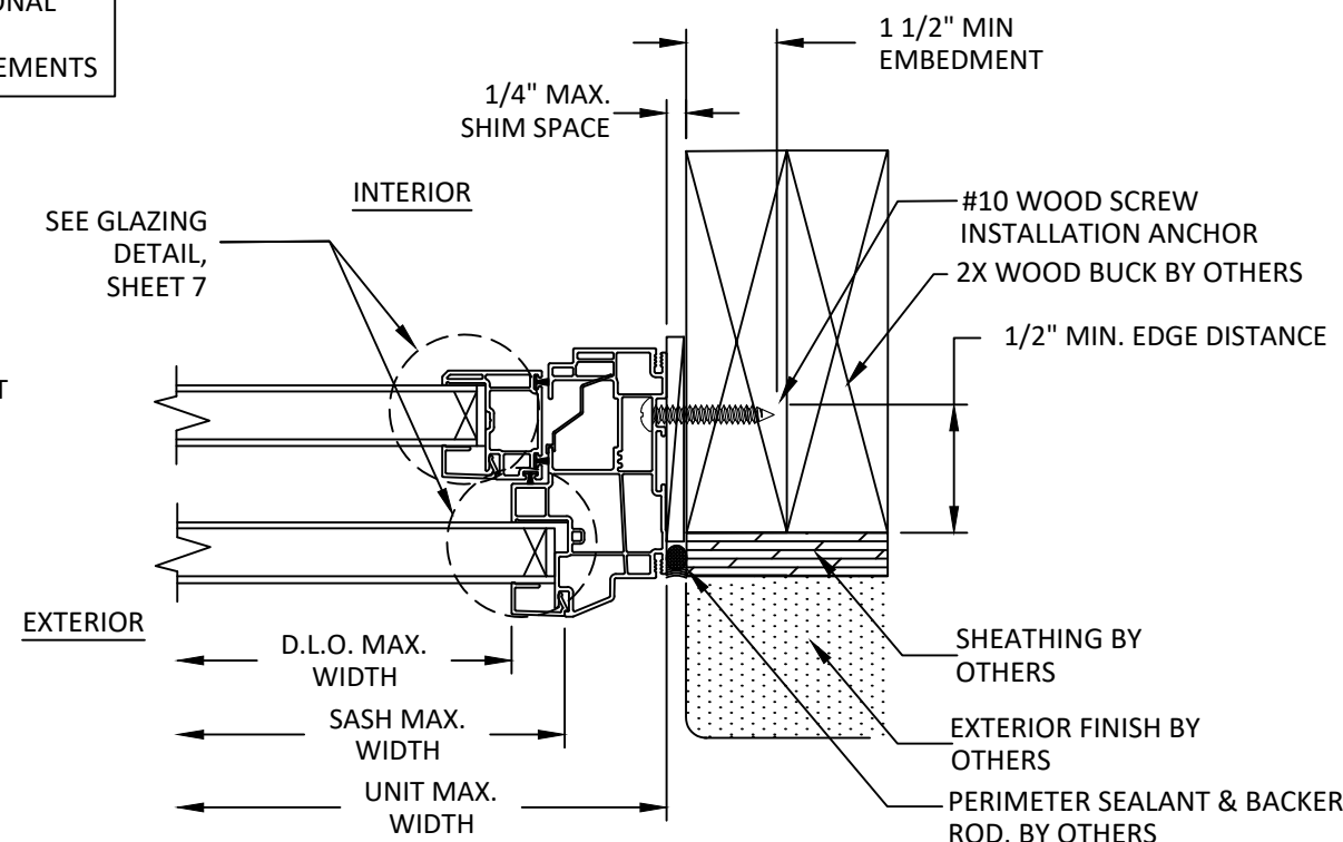
D 5 HORIZONTAL SECTION THROUGH FRAME INSTALLATION WOOD SUBSTRATE
