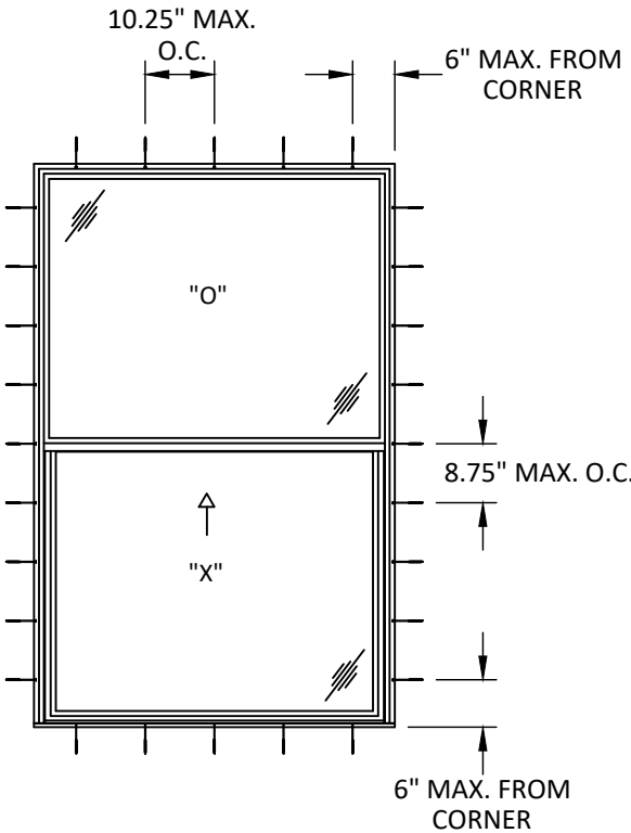
ANCHOR LAYOUT CLIP OR THROUGH FRAME INSTALLATION
