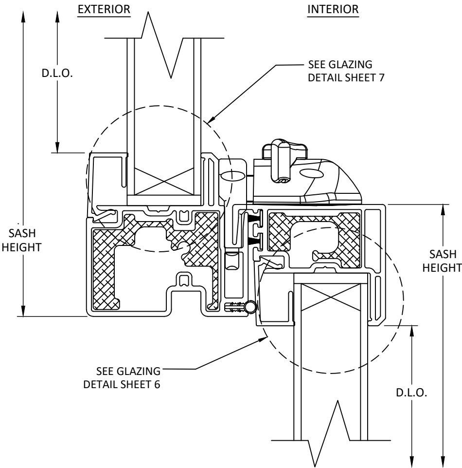
A 7 VERTICAL SECTION MEETING RAIL
