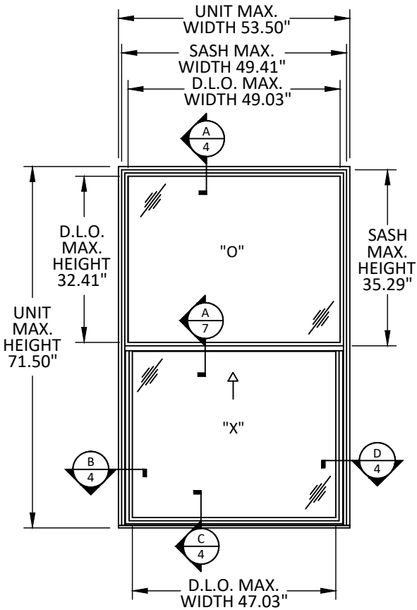
TYPICAL ELEVATION SINGLE HUNG EQUAL
