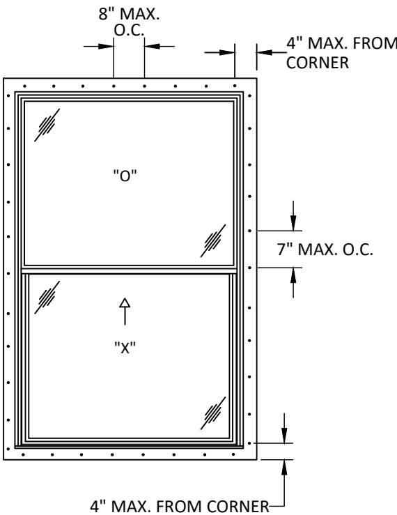
ANCHOR LAYOUT NAIL FIN INSTALLATION
