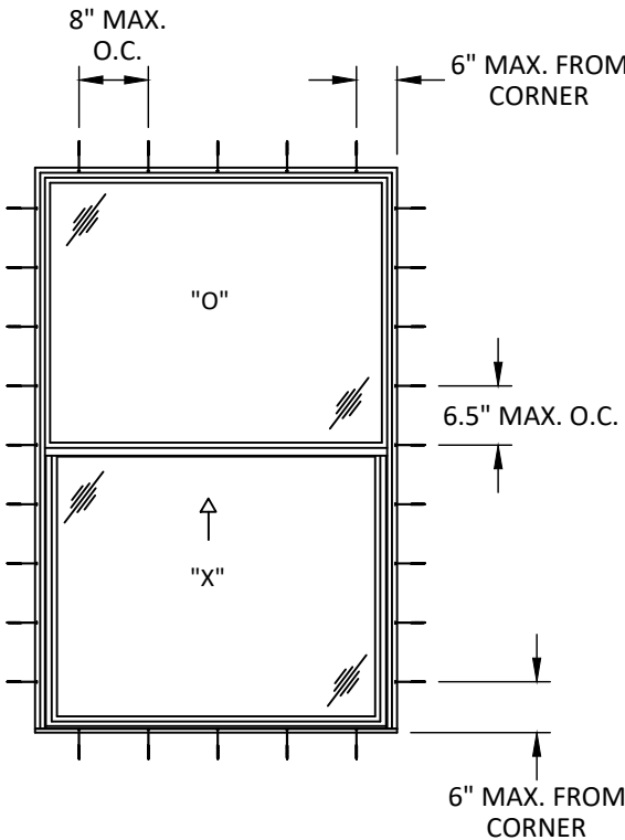
ANCHOR LAYOUT CLIP OR THROUGH FRAME INSTALLATION
