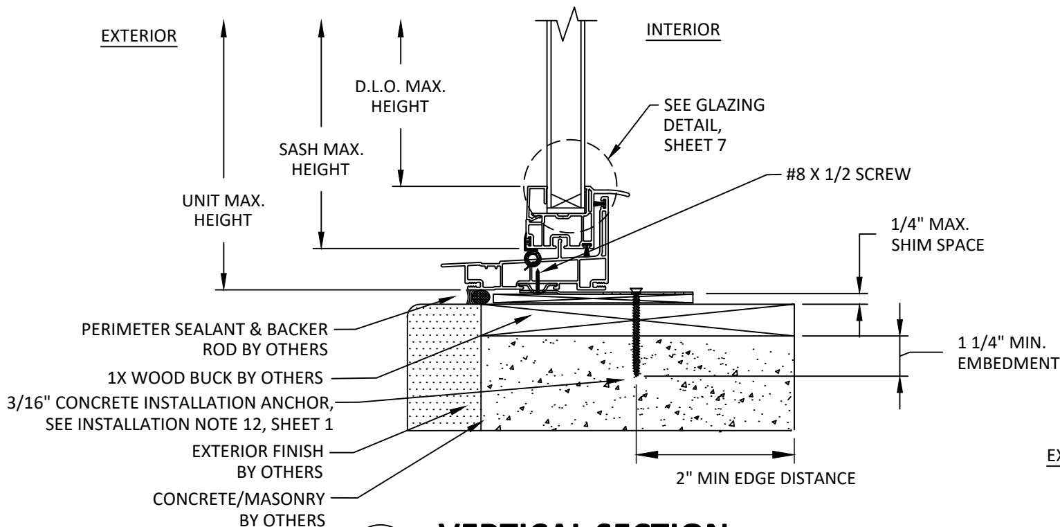
C 6 VERTICAL SECTION CLIP INSTALLATION CMU/CONCRETE
