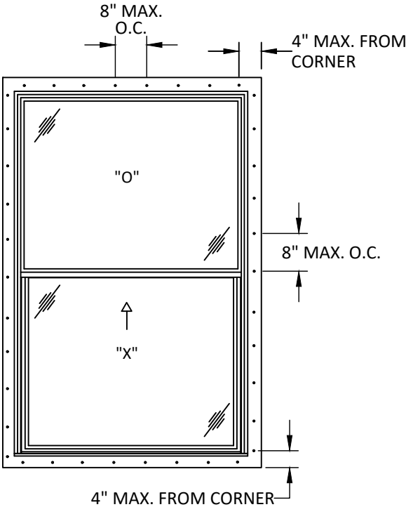
ANCHOR LAYOUT NAIL FIN INSTALLATION
