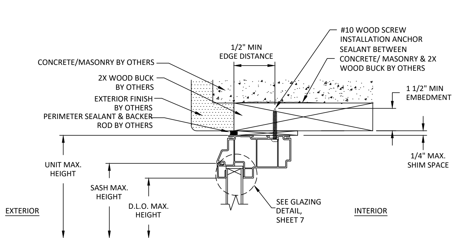
A 5 VERTICAL SECTION THROUGH FRAME INSTALLATION WOOD SUBSTRATE
