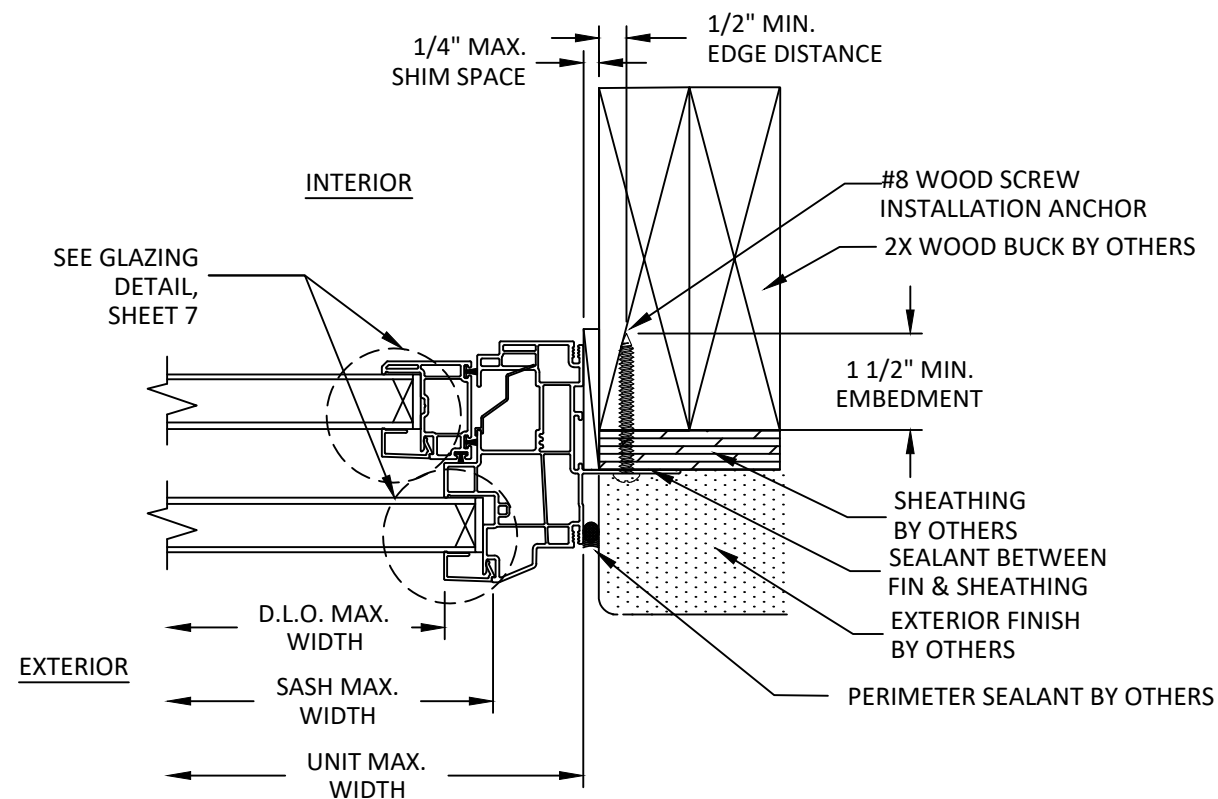
D 4 HORIZONTAL SECTION NAIL FIN INSTALLATION WOOD SUBSTRATE
