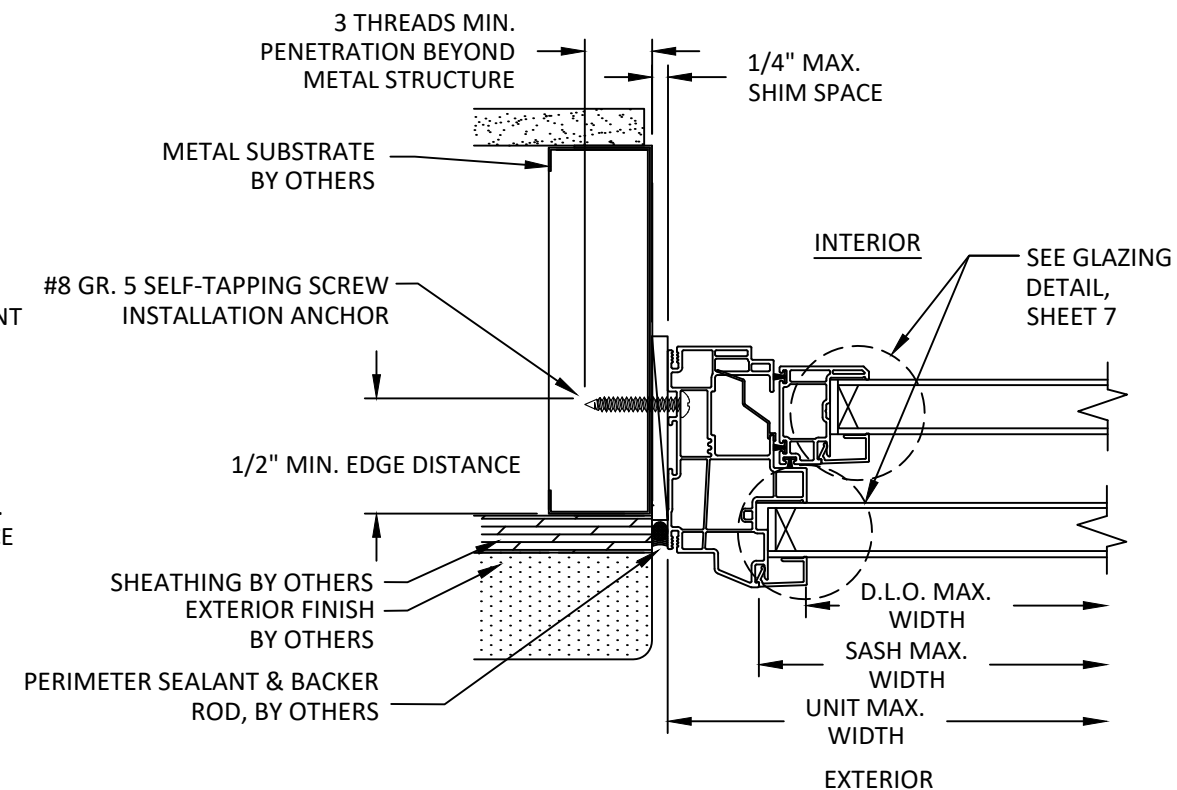
B 5 HORIZONTAL SECTION THROUGH FRAME INSTALLATION METAL SUBSTRATE
